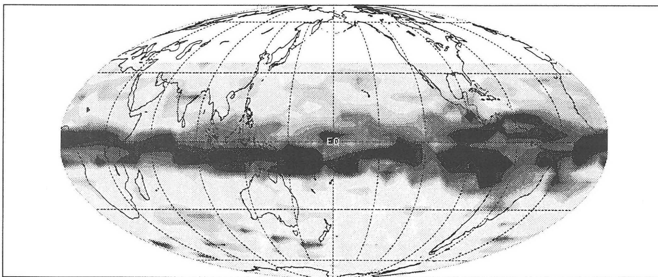
Sulfur dioxide near 25 kilometers (15 miles) altitude from the eruption of Mt. Pinatubo as observed by the Goddard managed Upper Atmosphere Research Satellite (UARS) on September 21, 1991. The volcanic plume appears as a belt of high concentration (dark areas) in the tropics.
